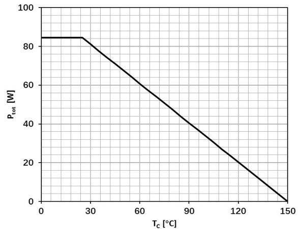
Figure 10 Power dissipation
