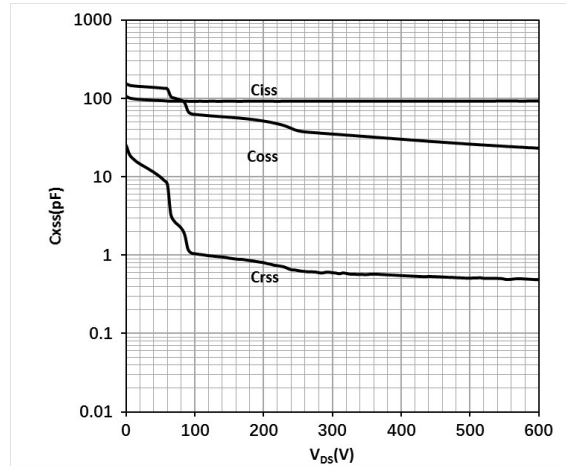
Figure 14 Typ. capacitances
