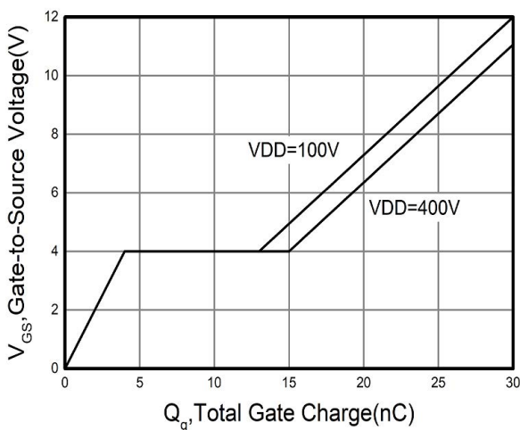
Q_g , Total Gate Charge (nC) Figure 5. Gate Charge
