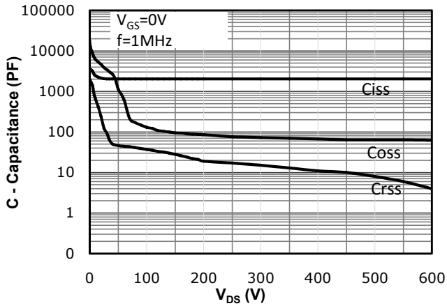
Fig 11: Capacitance Characteristics
