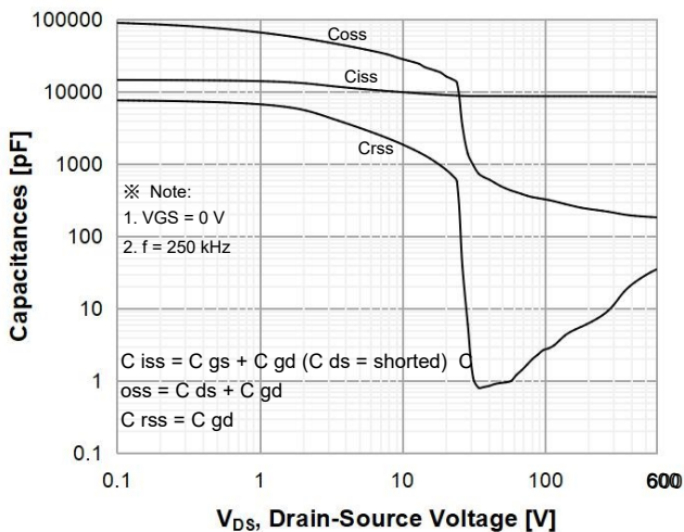
Figure 5. Capacitance Characteristics
