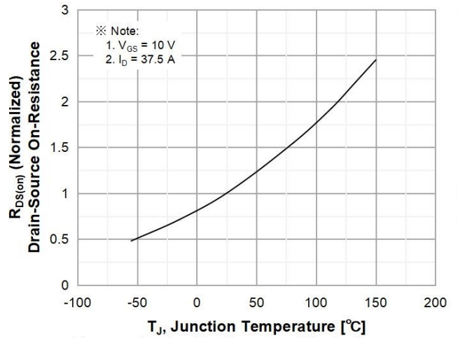
Figure 8. On-Resistance Variation
