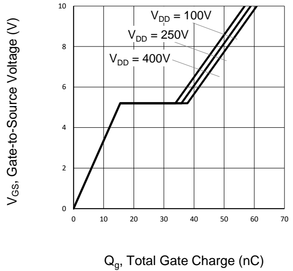
Figure 8. Gate Charge
