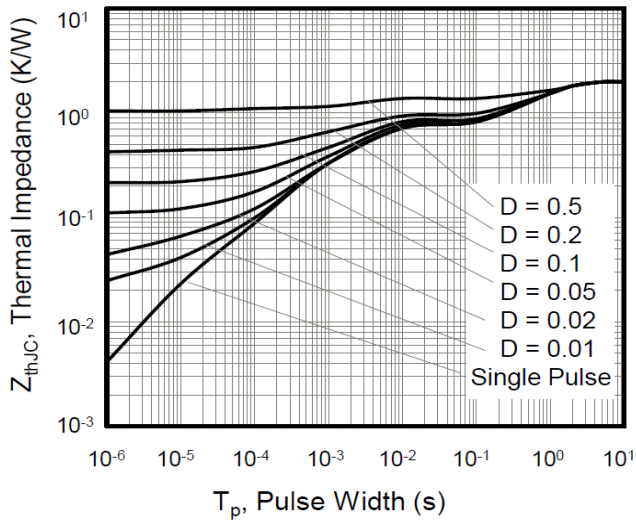
Figure 7. Transient Thermal Impedance (TO-220F)
